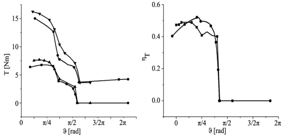
Figure 9: Left Side, the Predicted and Measured Torque [Nm] vs the Rotation \theta [rad] for Cam Pair B. Up Triangle, Lower Triangle, Square and Circle Represent, Respectively, T_{c,m} , T_{s,m} , T_{s,th} and T_{c,th} . Right Side, the Efficiency \eta_T vs the Rotation \theta [rad]. Square and Circle Represent, Respectively, Theoretical Efficiency and Measured.
