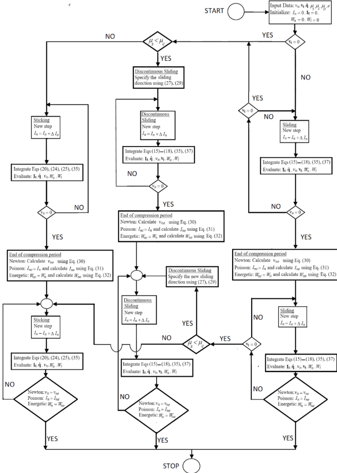
Figure 1: Numerical Procedure for the Solution of the Three-Dimensional Systems
